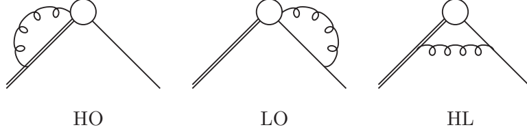
Figure 1. Diagrams evaluated to determine the renormalisation constant Z_{\pm} using a two-parton external state (the two letters describe the ends of the gluon line: Heavy quark, Light quark or Operator, i.e. the path-ordered exponential).
