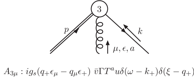
Figure 2. The three leading-order contributions to the matrix element of O_{\pm} with a three-parton external state.
