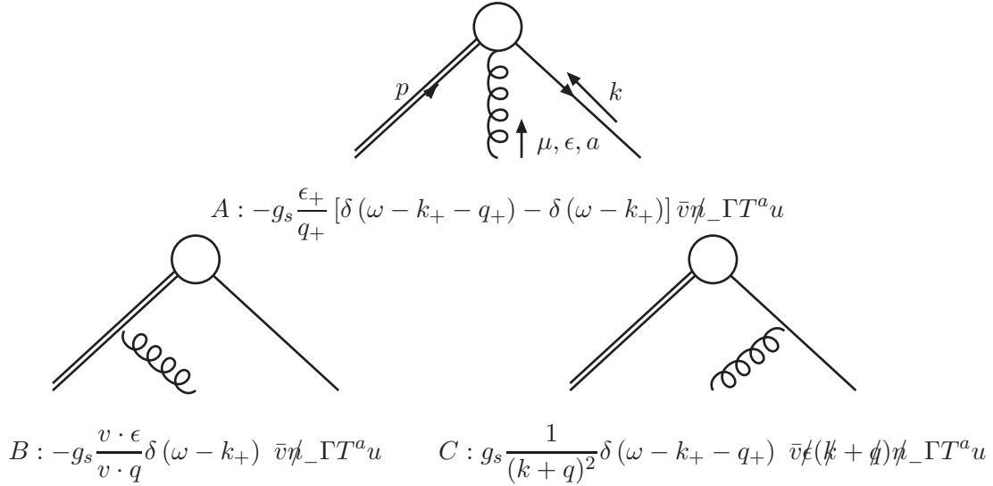
Figure 2. The three leading-order contributions to the matrix element of O_{\pm} with a three-parton external state.
